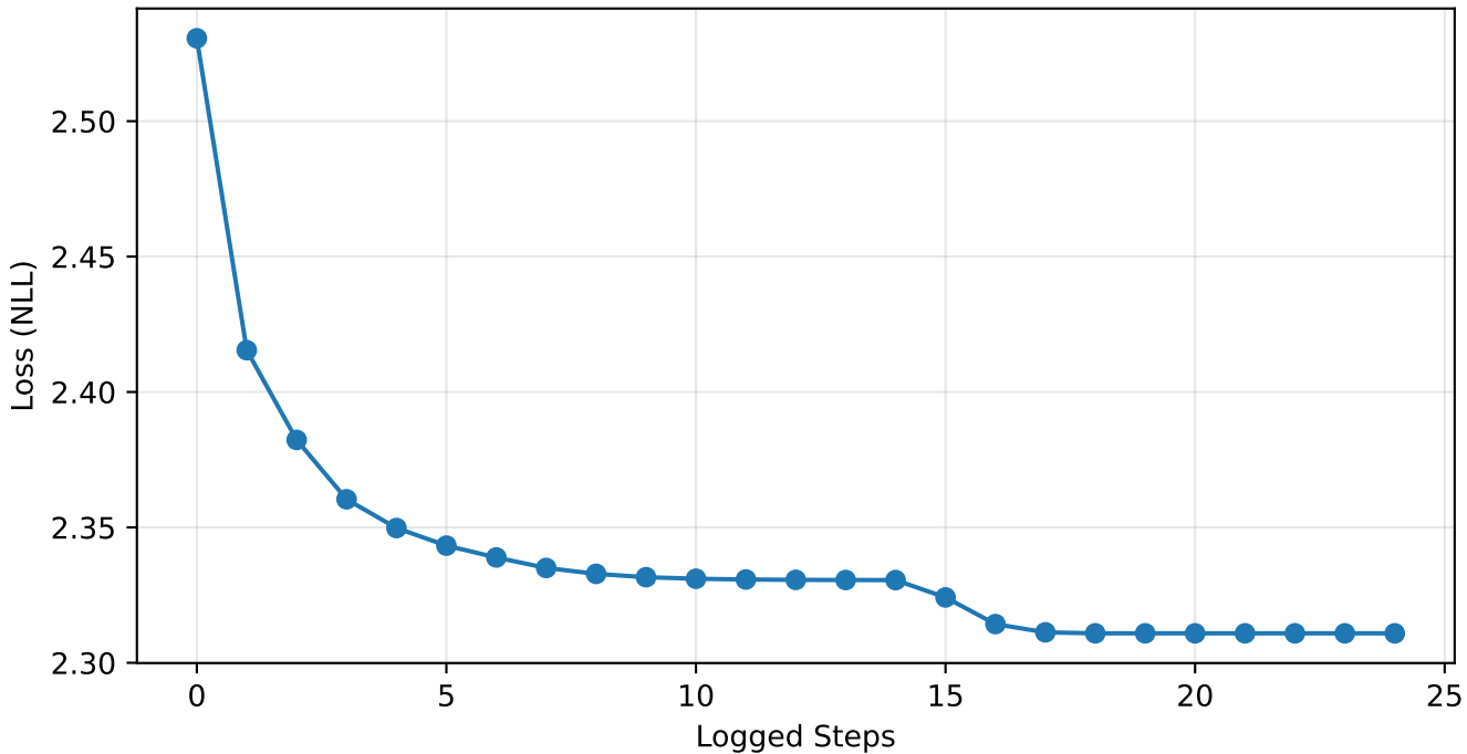
Optimization Loss Curve | gw190425_phenompnrt-hs_posterior
