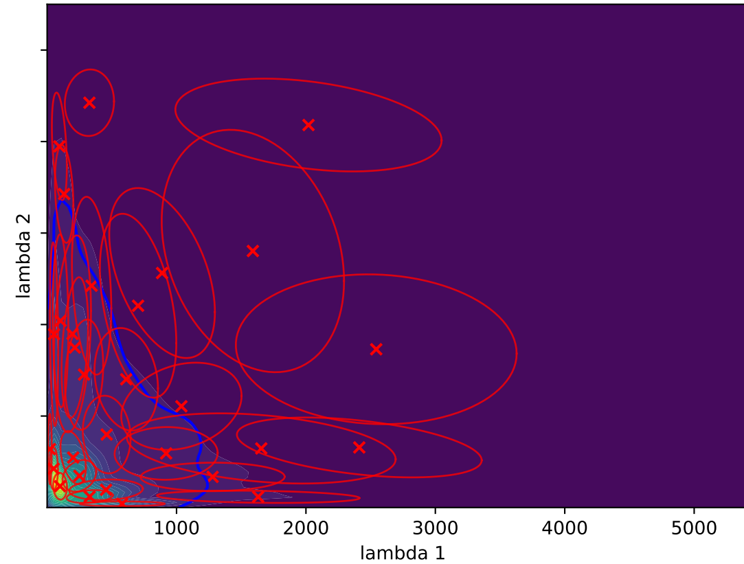
Gaussian Splat (L-BFGS) D_{KL}(P||Q) = -0.0948
