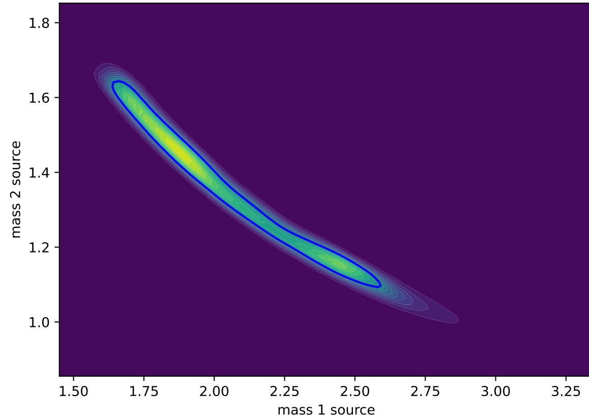
Original KDE (mass 1 source vs mass 2 source)
