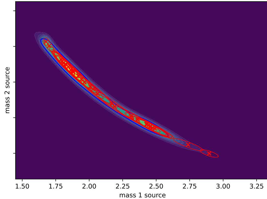
Gaussian Splat (L-BFGS) D_{\text{KL}}(P||Q) = 0.0016
