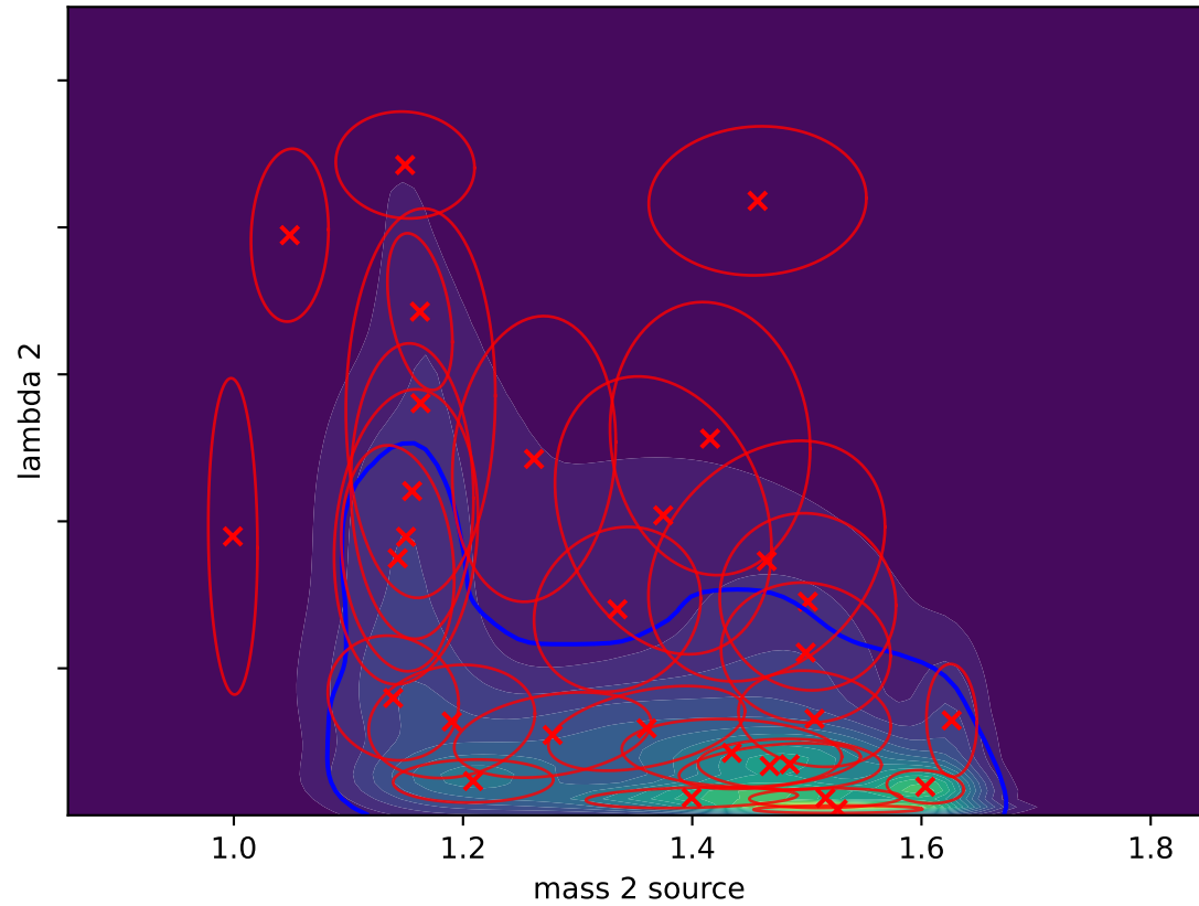
Gaussian Splat (L-BFGS) D_{\text{KL}}(P||Q) = -0.0256
