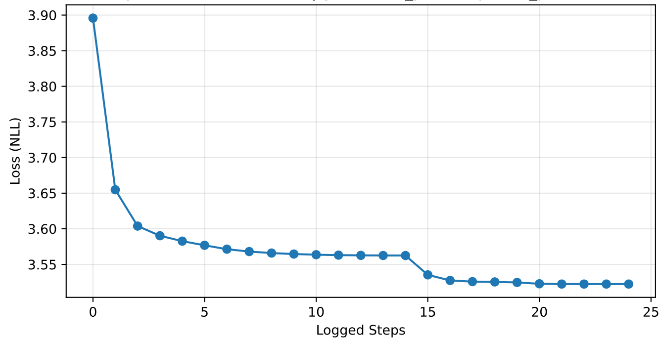
Optimization Loss Curve | gw190425_phenompnr-1s_posterior
