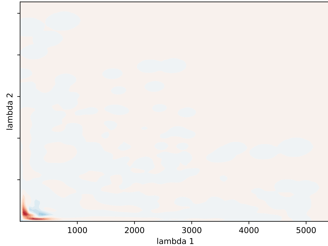
Probability Residual (P - Q)
