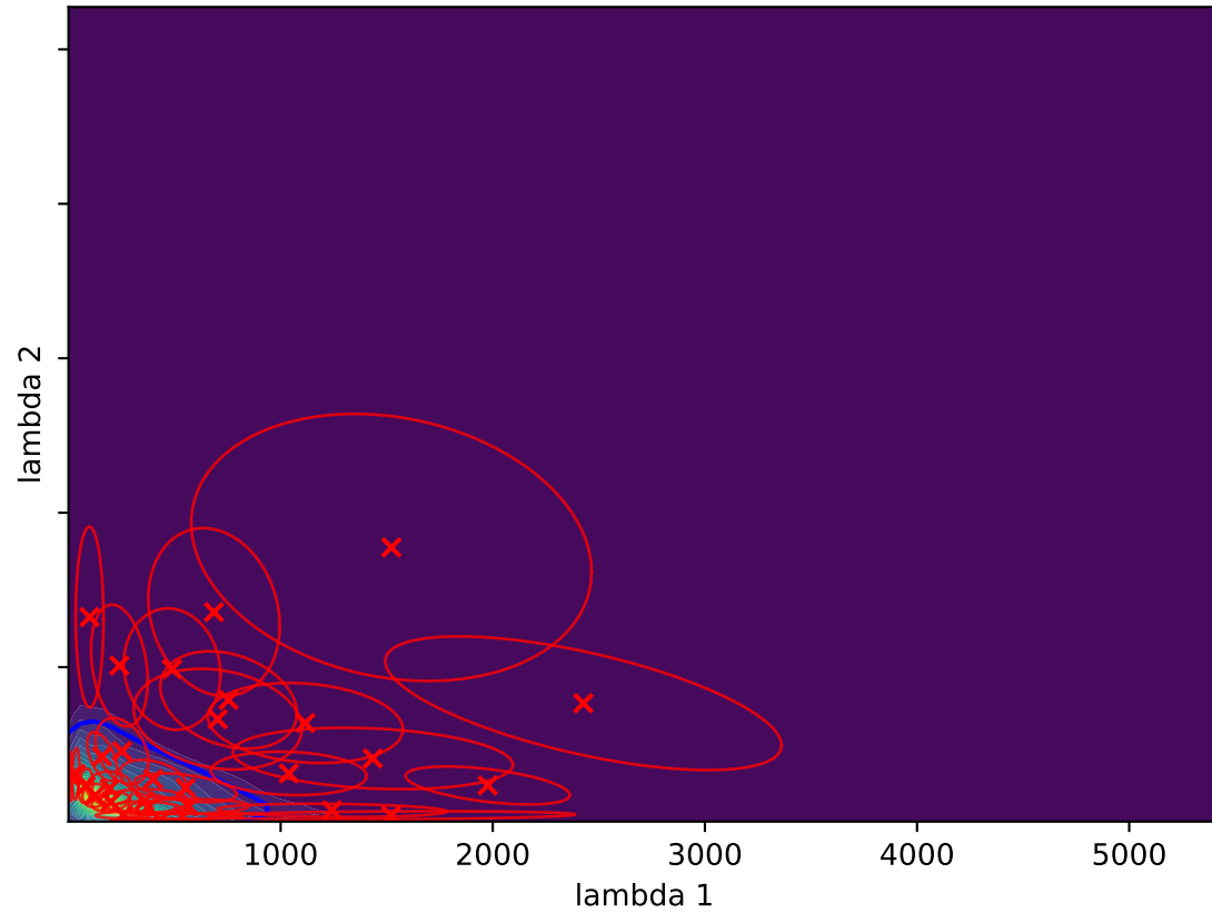
Gaussian Splat (L-BFGS) D_{\text{KL}}(P||Q) = -0.1183
