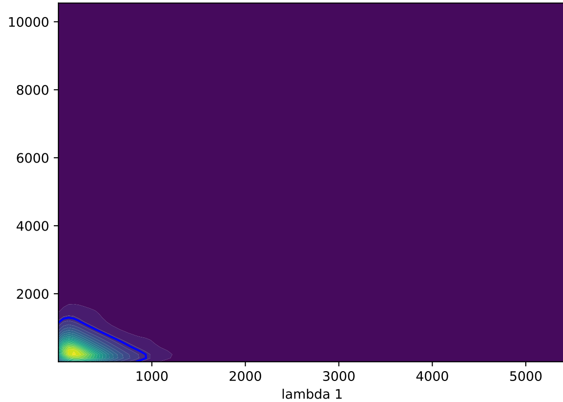
Original KDE (lambda 1 vs lambda 2)
