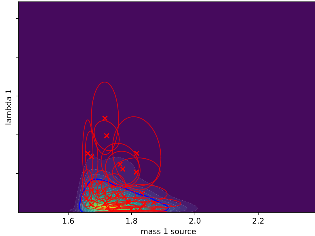
Gaussian Splat (L-BFGS) D_{KL}(P||Q) = -0.0550
