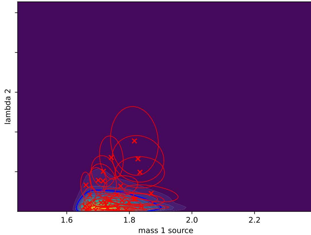
Gaussian Splat (L-BFGS) D_{KL}(P||Q) = -0.0575
