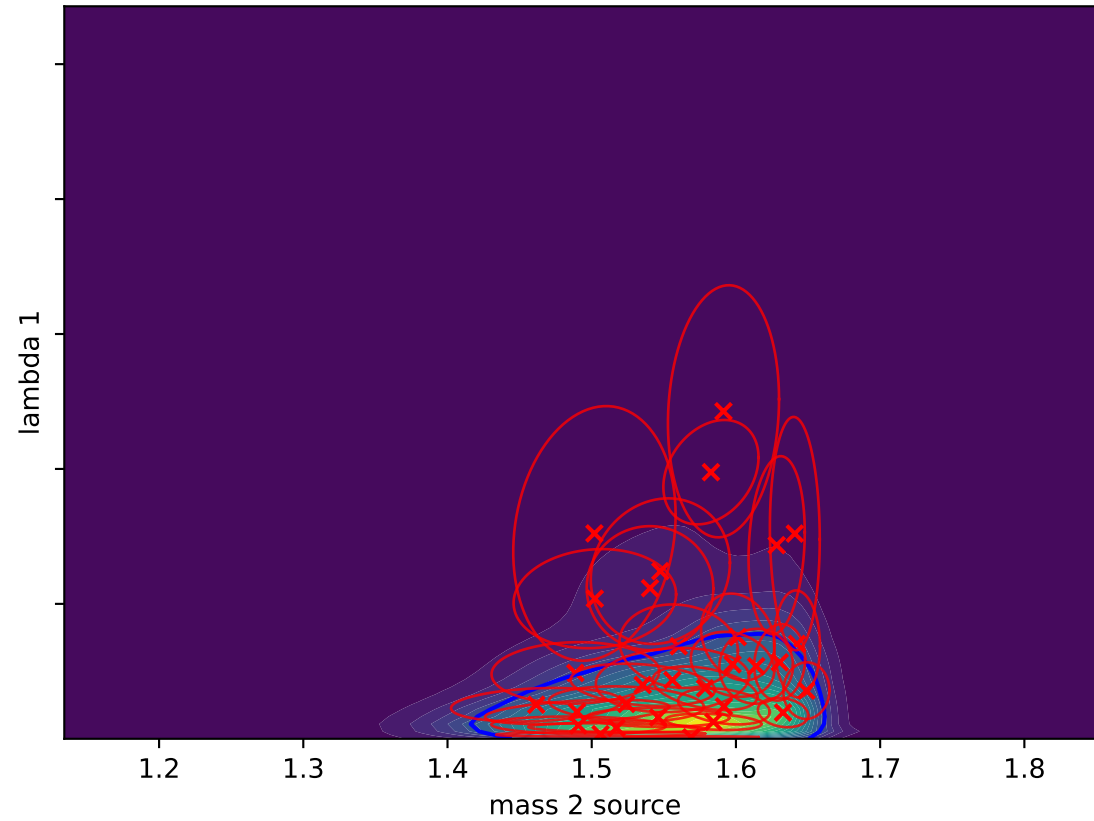
Gaussian Splat (L-BFGS) D_{KL}(P||Q) = -0.0597
