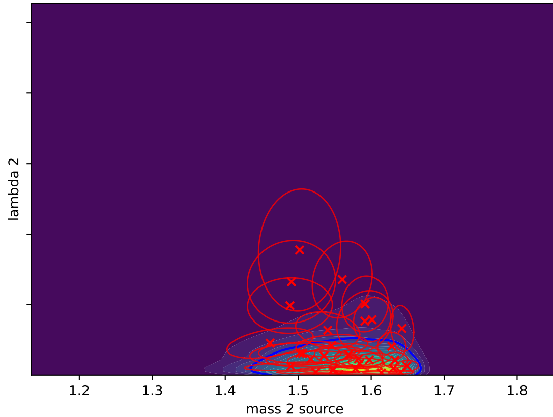
Gaussian Splat (L-BFGS) D_{KL}(P||Q) = -0.0577
