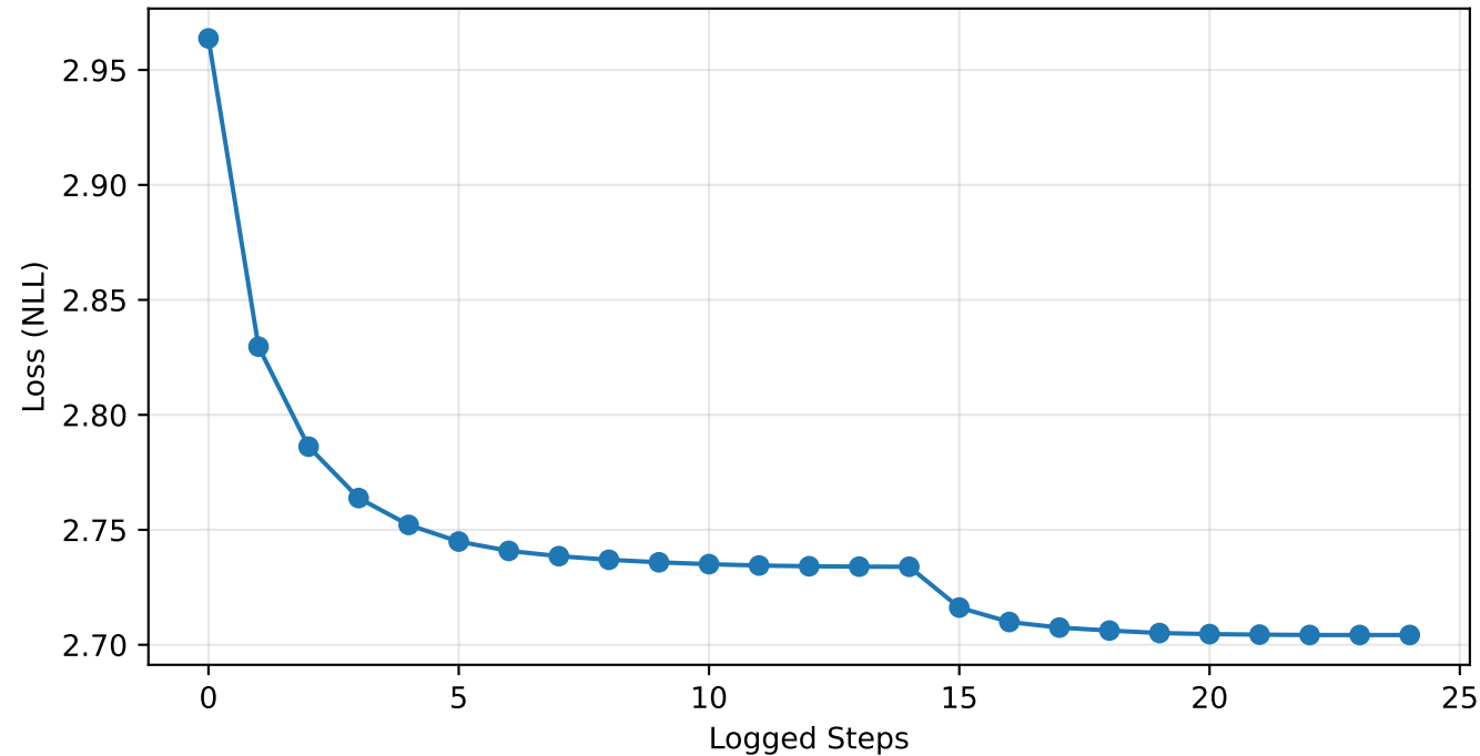
Optimization Loss Curve | gw190425_taylorf2-hs_posterior
