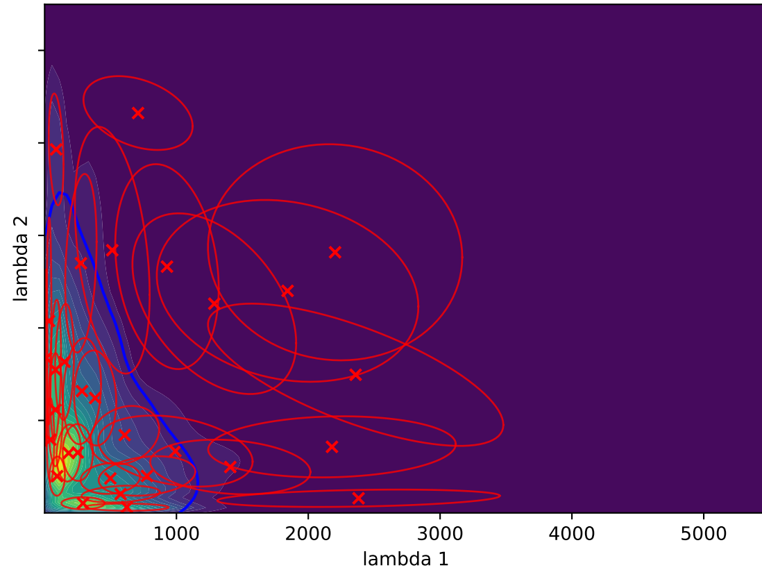
Gaussian Splat (L-BFGS) D_{KL}(P||Q) = -0.1442
