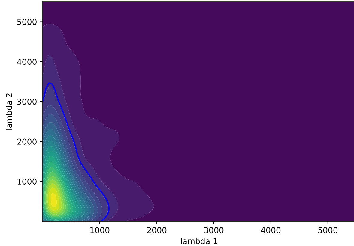
Original KDE (lambda 1 vs lambda 2)
