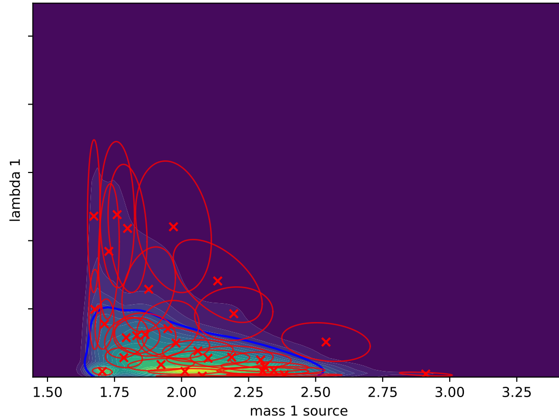
Gaussian Splat (L-BFGS) D_{KL}(P||Q) = -0.1147
