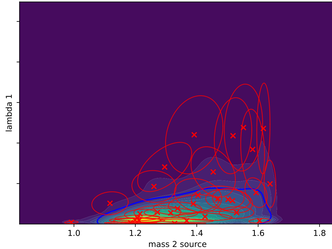
Gaussian Splat (L-BFGS) D_{KL}(P||Q) = -0.1052
