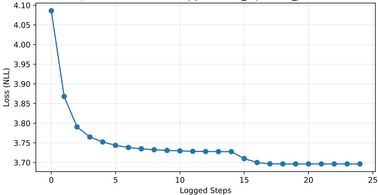
Optimization Loss Curve | gw190425_taylorf2-ls_posterior
