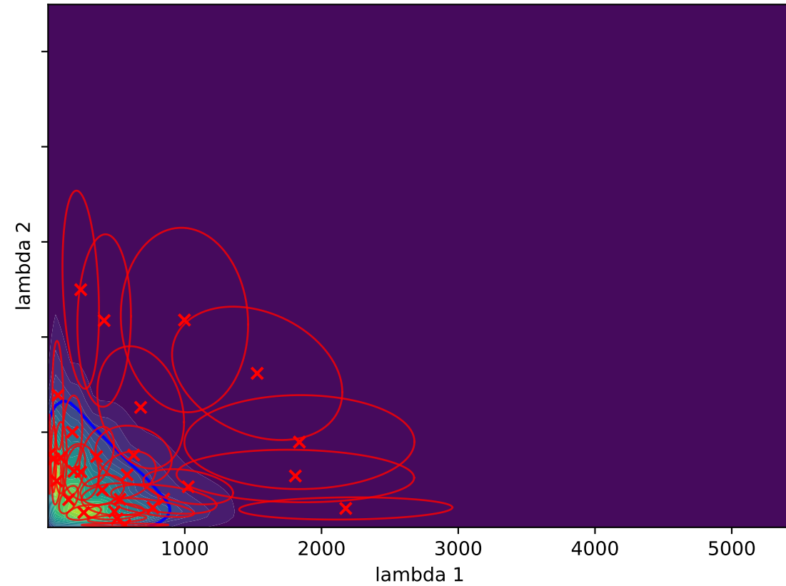
Gaussian Splat (L-BFGS) D_{KL}(P||Q) = -0.1058
