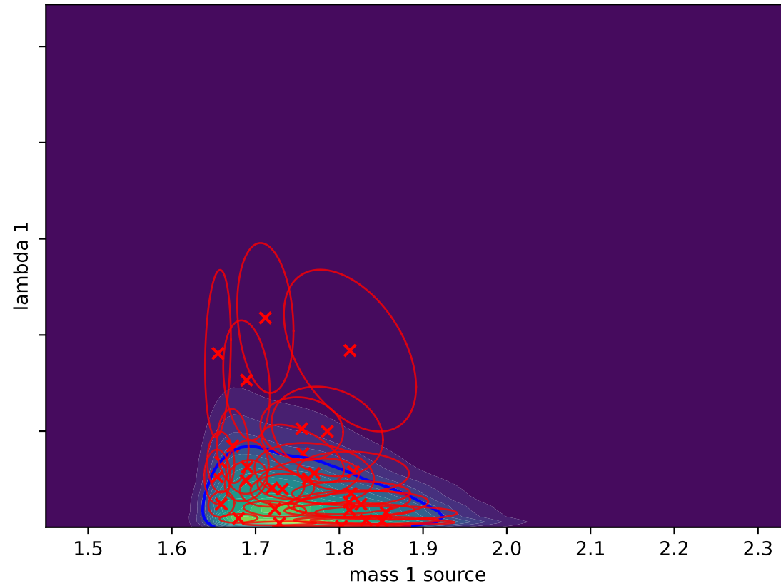
Gaussian Splat (L-BFGS) D_{KL}(P||Q) = -0.0610
