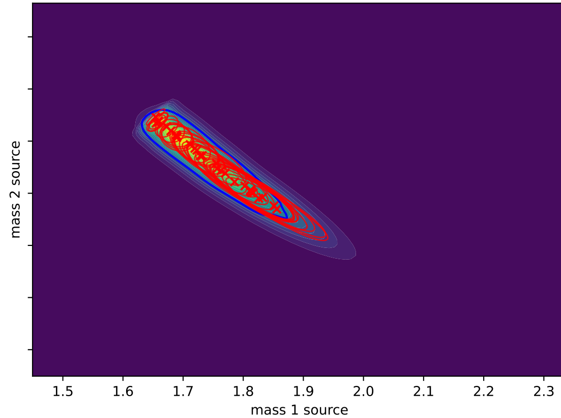
Gaussian Splat (L-BFGS) D_{\text{KL}}(P||Q) = -0.0039
