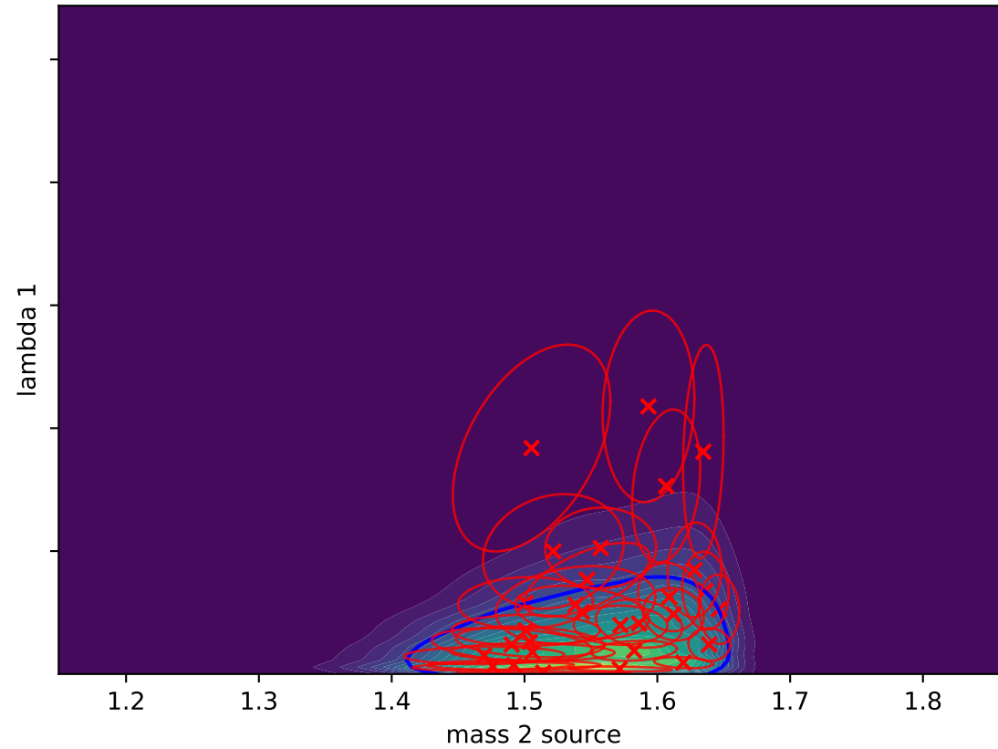
Gaussian Splat (L-BFGS) D_{KL}(P||Q) = -0.0628
