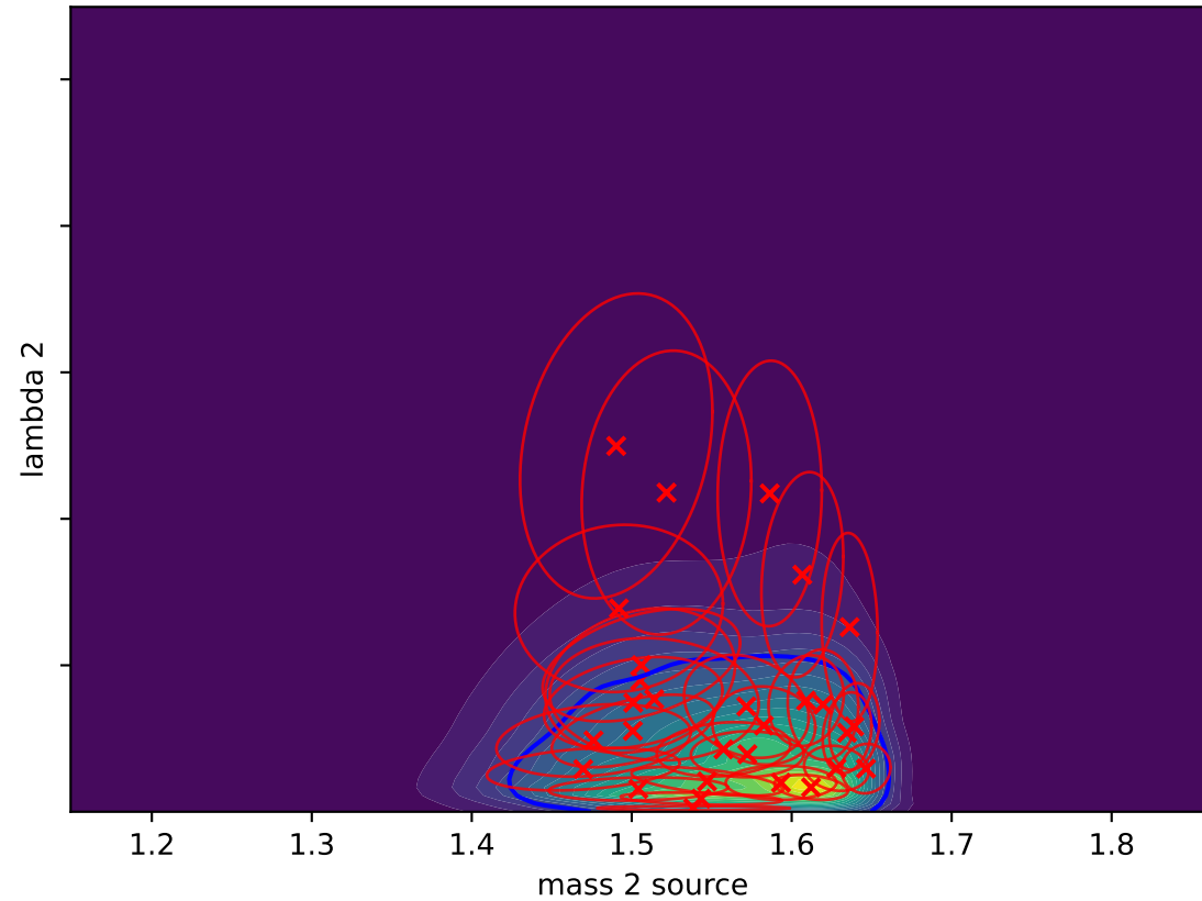
Gaussian Splat (L-BFGS) D_{KL}(P||Q) = -0.0438
