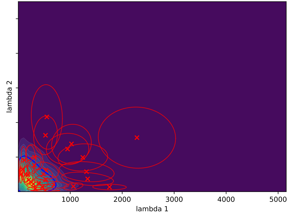
Gaussian Splat (L-BFGS) D_{KL}(P||Q) = -0.0603
