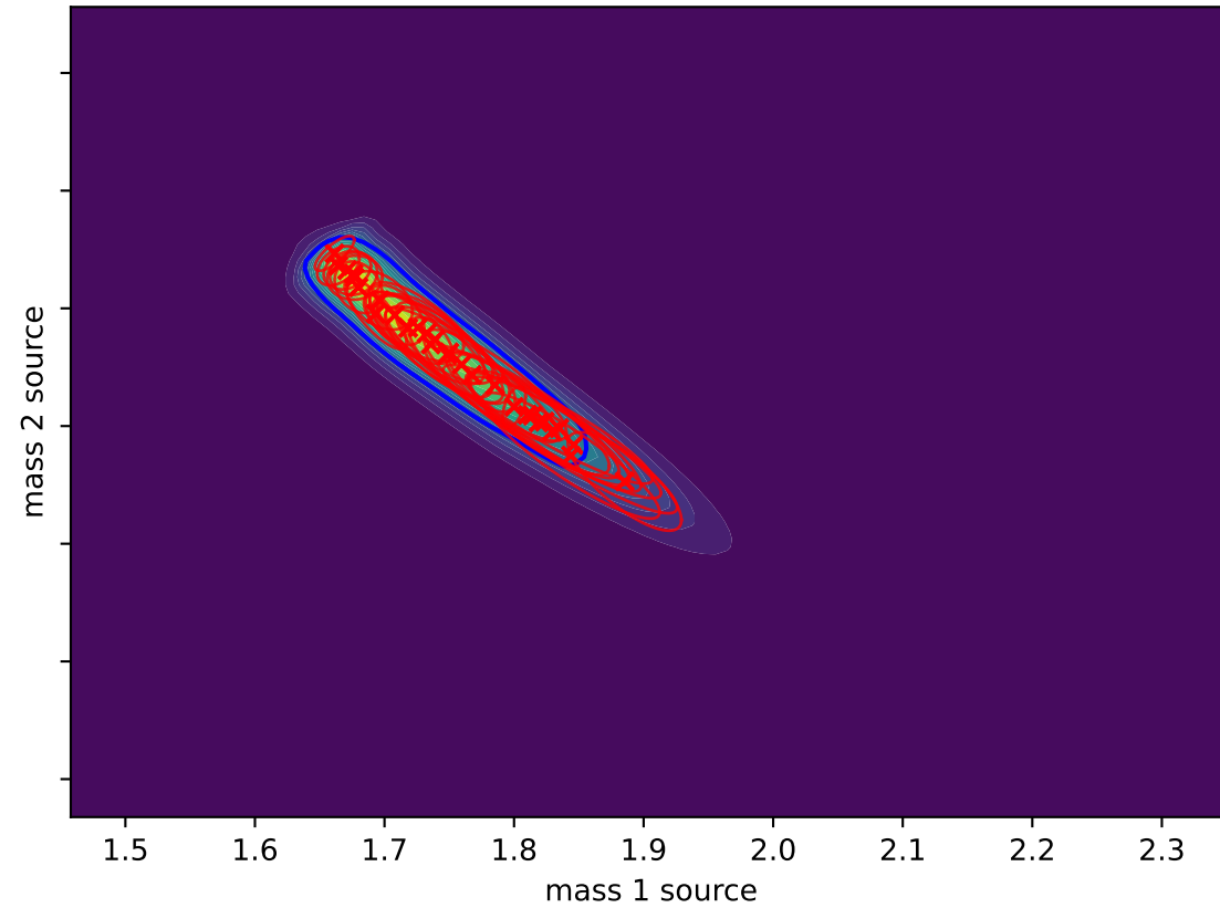
Gaussian Splat (L-BFGS) D_{\text{KL}}(P||Q) = 0.0074
