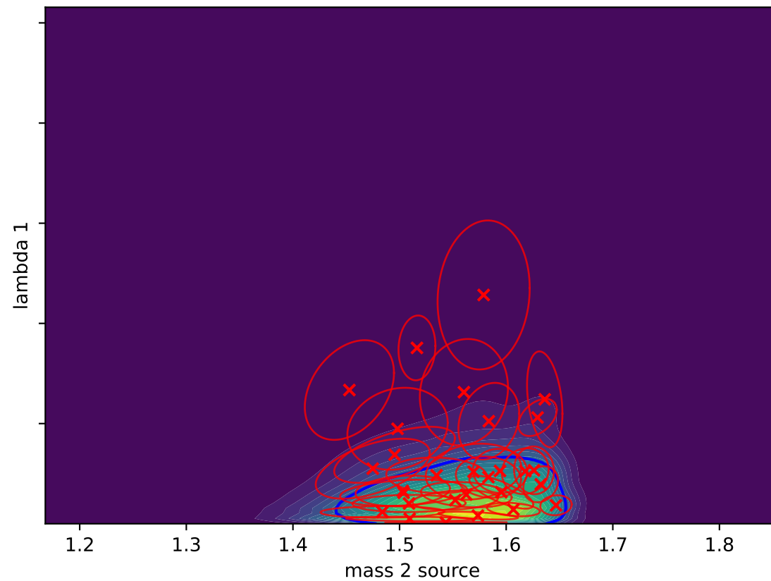
Gaussian Splat (L-BFGS) D_{KL}(P||Q) = -0.0390
