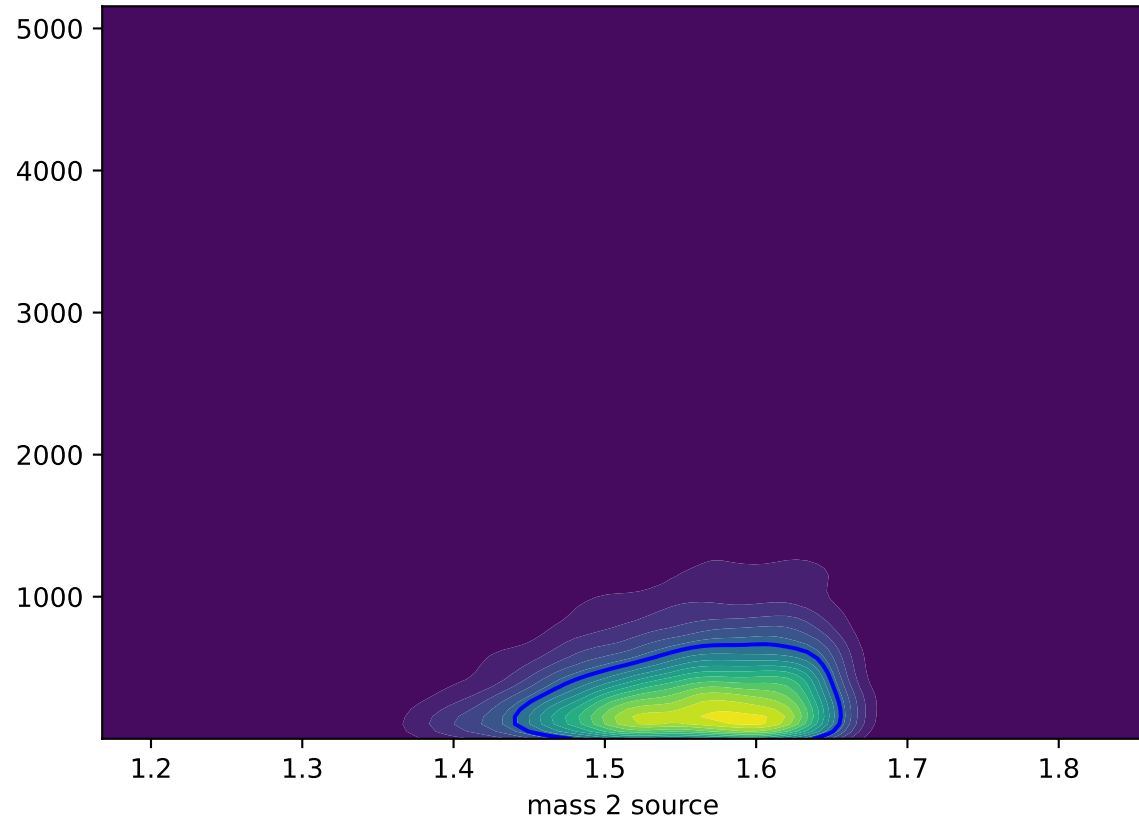
Original KDE (mass 2 source vs lambda 1)
