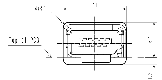
Reference Dimensions of Panel Cutout (Free)
