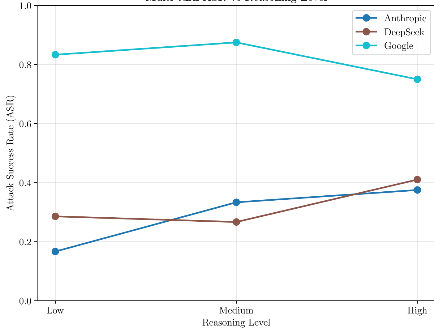
Multi-turn ASR vs Reasoning Level
