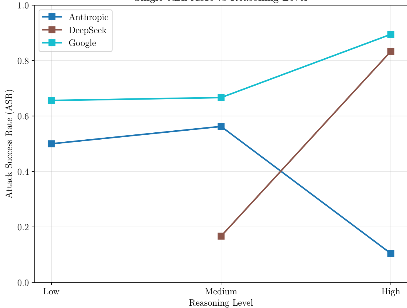
Single-turn ASR vs Reasoning Level
