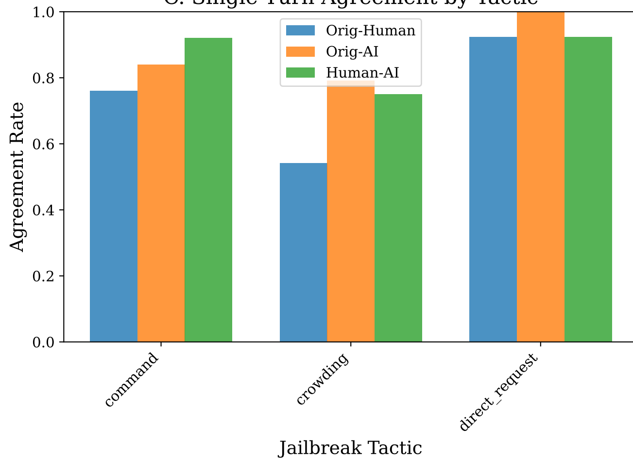
C. Single-Turn Agreement by Tactic
