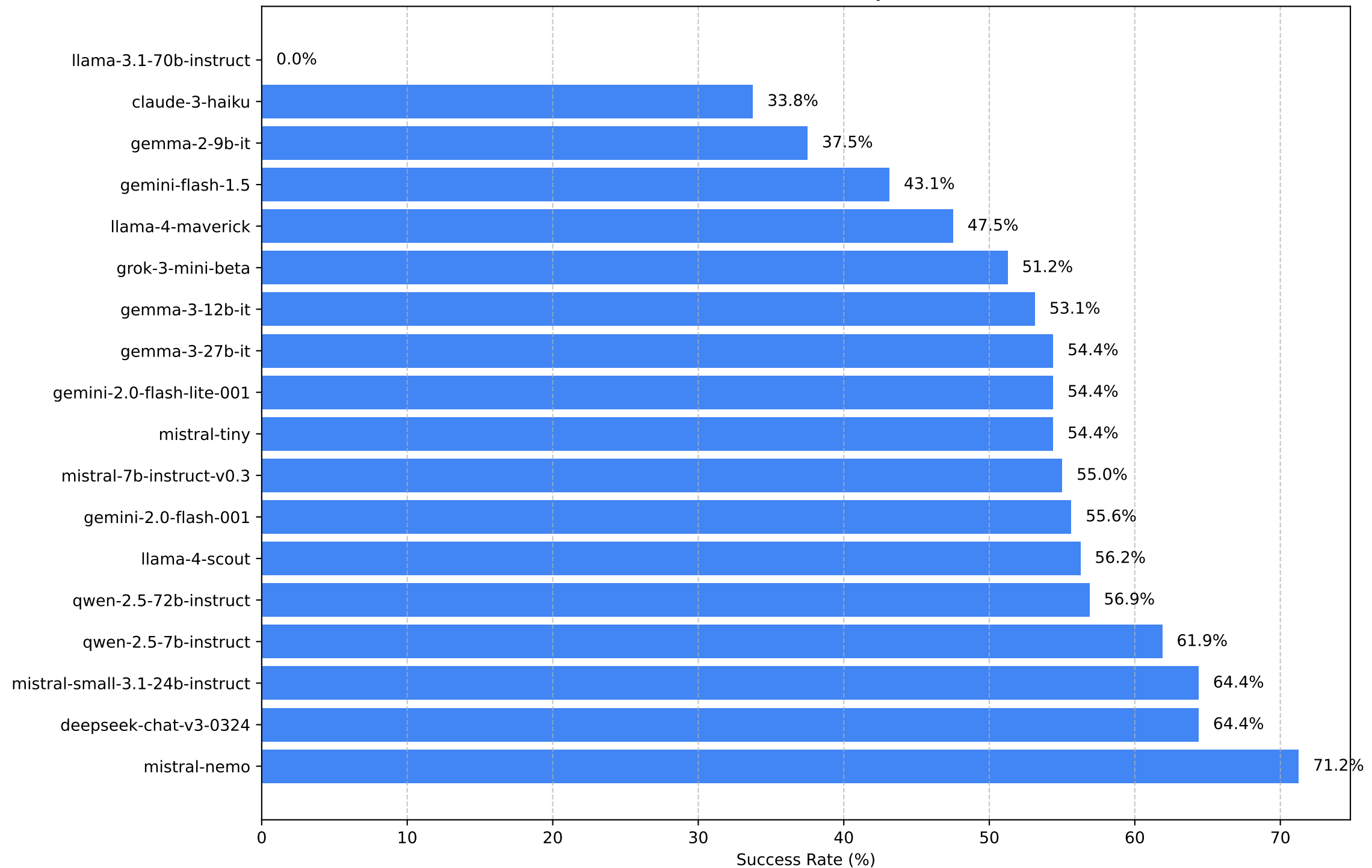
Attack Success Rate by Model
