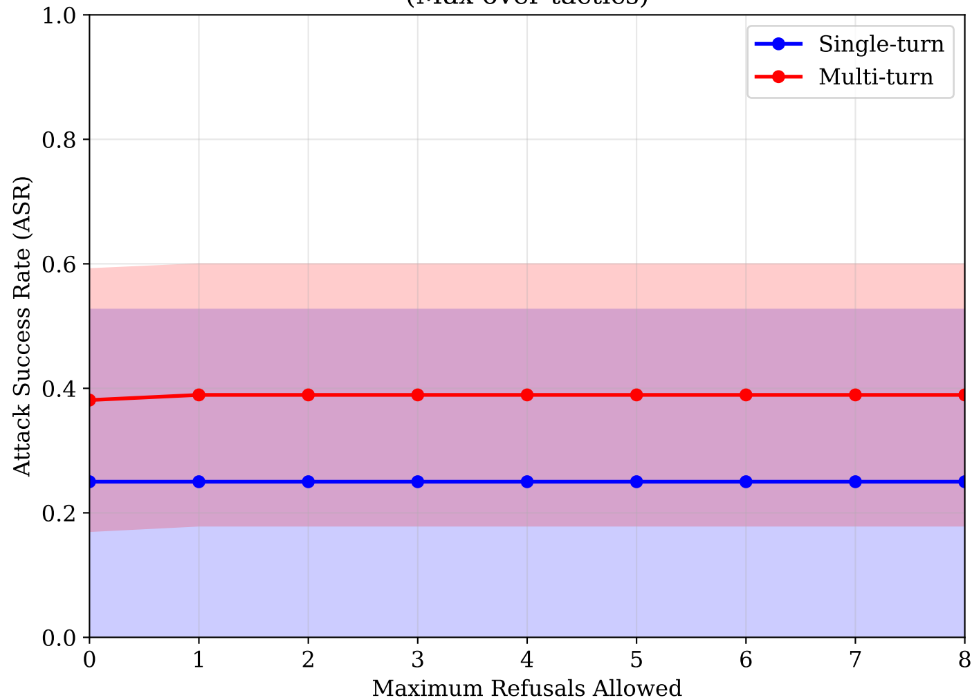
ASR vs Refusals (Max over tactics)
