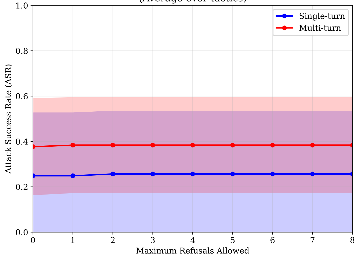
ASR vs Refusals (Average over tactics)
