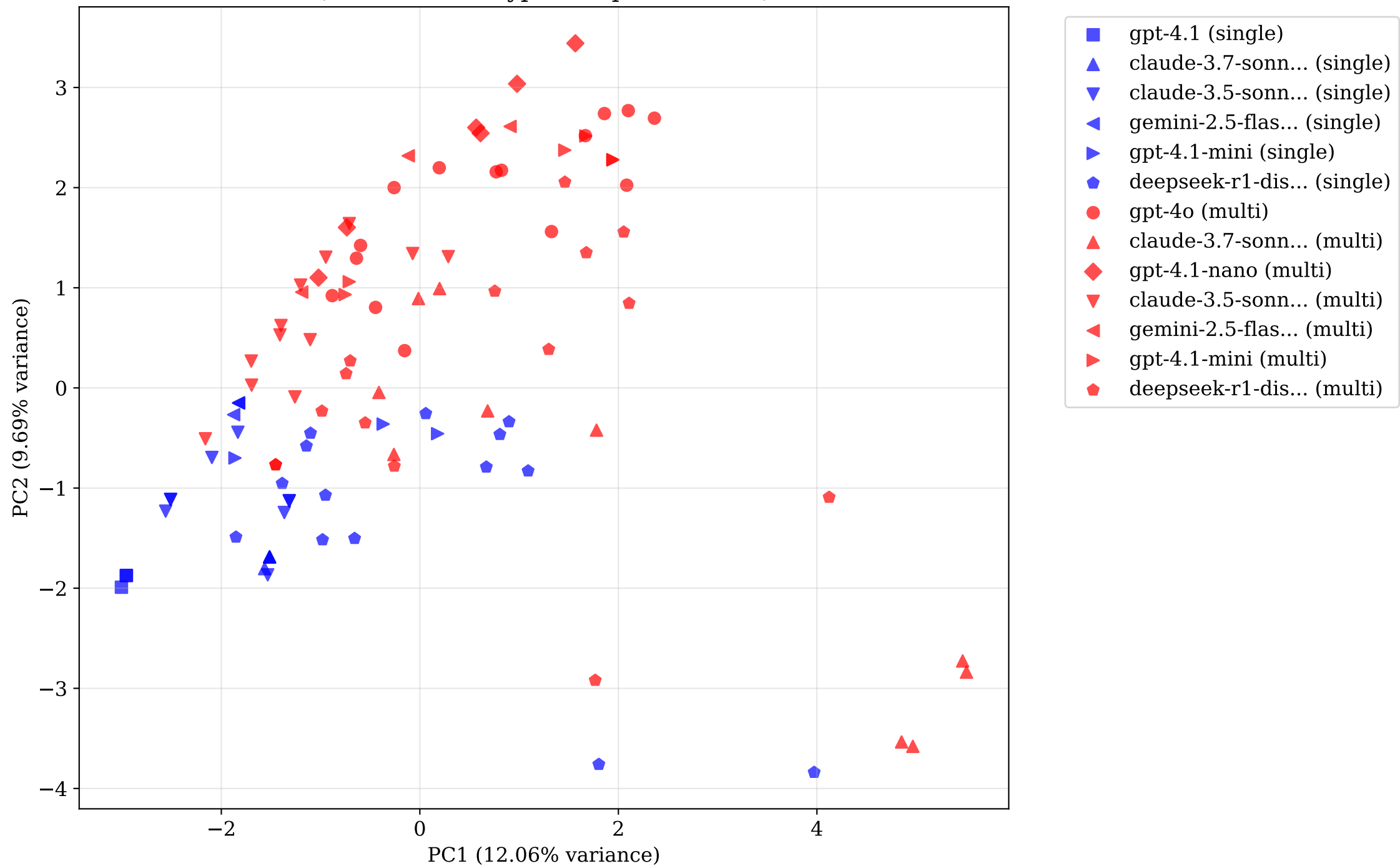
PCA: Models and Turn Types (Colors=Turn Type, Shapes=Models)
