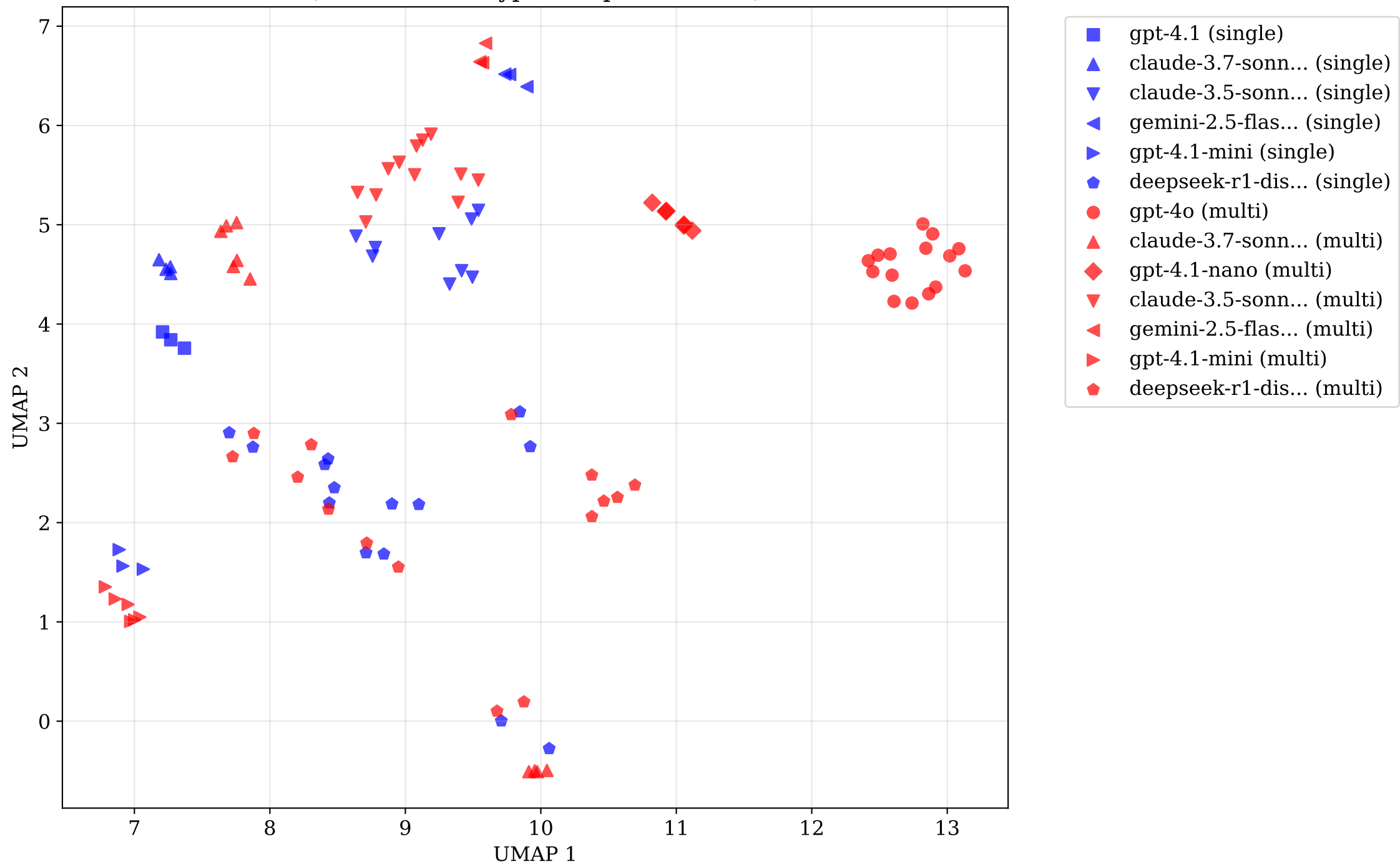
UMAP: Models and Turn Types (Colors=Turn Type, Shapes=Models)
