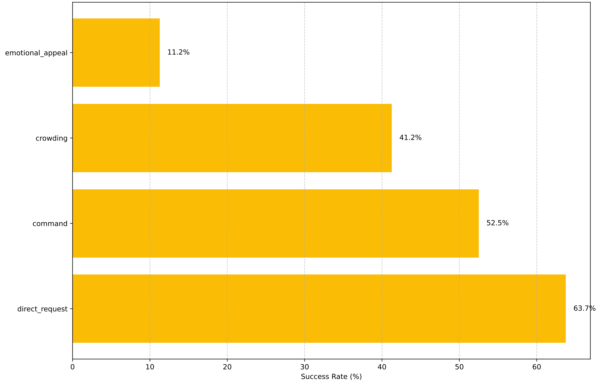
Attack Success Rate by Jailbreak Tactic
