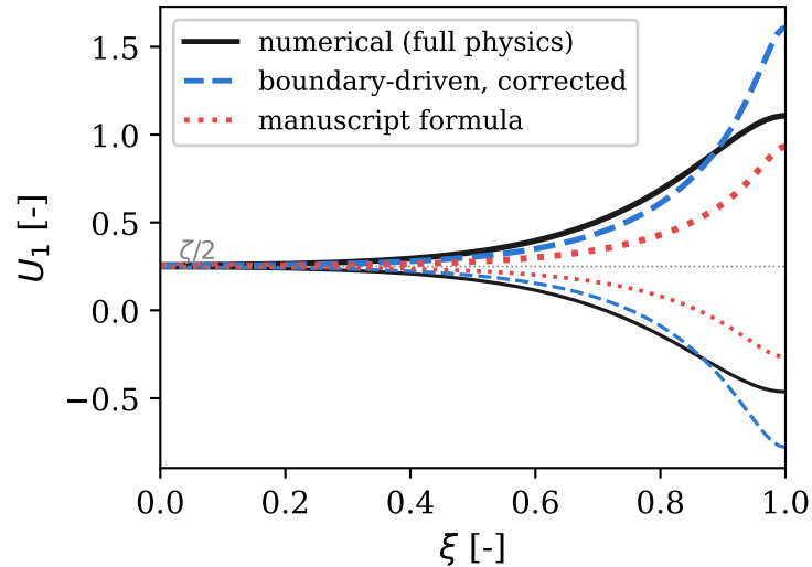
(b) First-order velocity U_1 thick: \eta = 0.46 ; thin: \eta = 0.06
