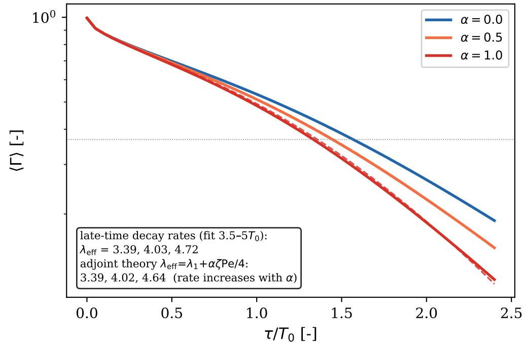
(c) SLR runs, local trapping zone solid: nonlinear; dashed: quasi-static ansatz; dotted: exact 1st-order
