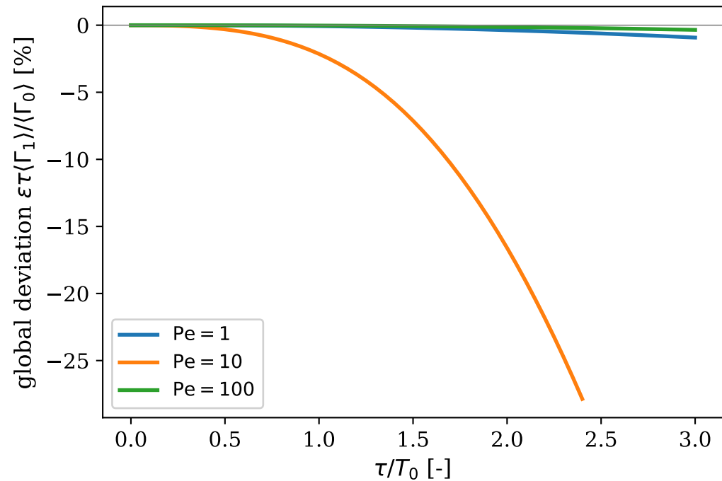
(a) Domain-averaged coupling effect, \varepsilon = 1 (negative: stronger coupling accelerates flushing, stretched clock)
