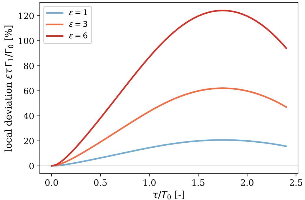
(b) Seaward trapping zone, Pe = 10 (positive: coupling retards local cleanup)
