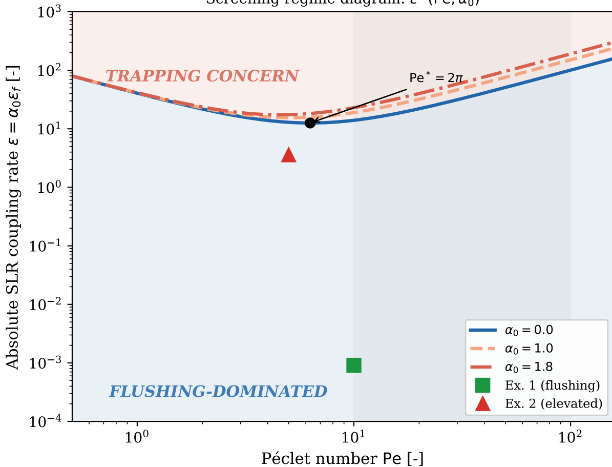
Screening regime diagram: \varepsilon^*(\text{Pe}, \alpha_0)
