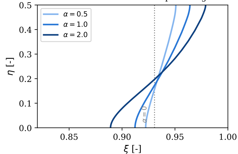
(a) Steady wedge: \chi = 0.5 isochlor (nonlinear) interface rotates about mid-depth as \alpha grows
