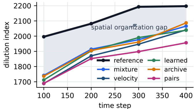
c Breakthrough-only selection favors velocity memory, not universal adequacy
