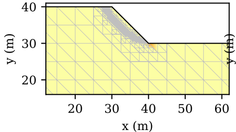
GI: \sqrt{J_2(\varepsilon^p)}/\max no colapso
