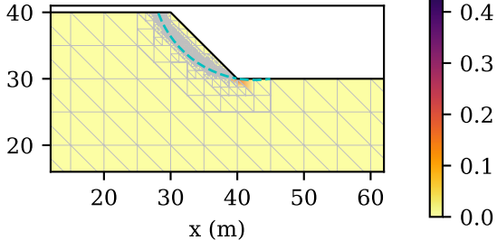
SRM: \sqrt{J_2(\varepsilon^p)}/\max no colapso
