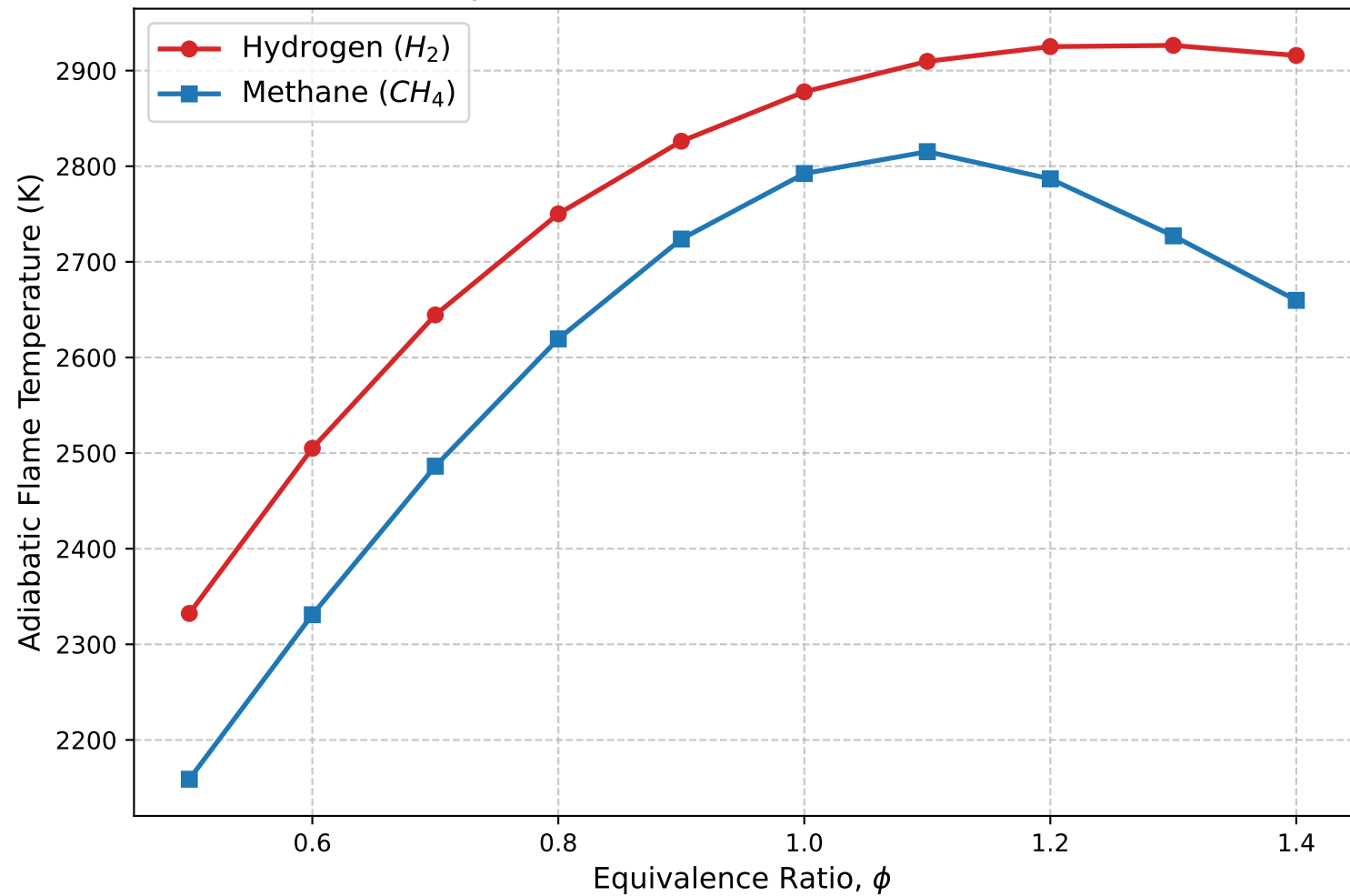
Complete Combustion T_{ad} at T_{in} = 1100 K
