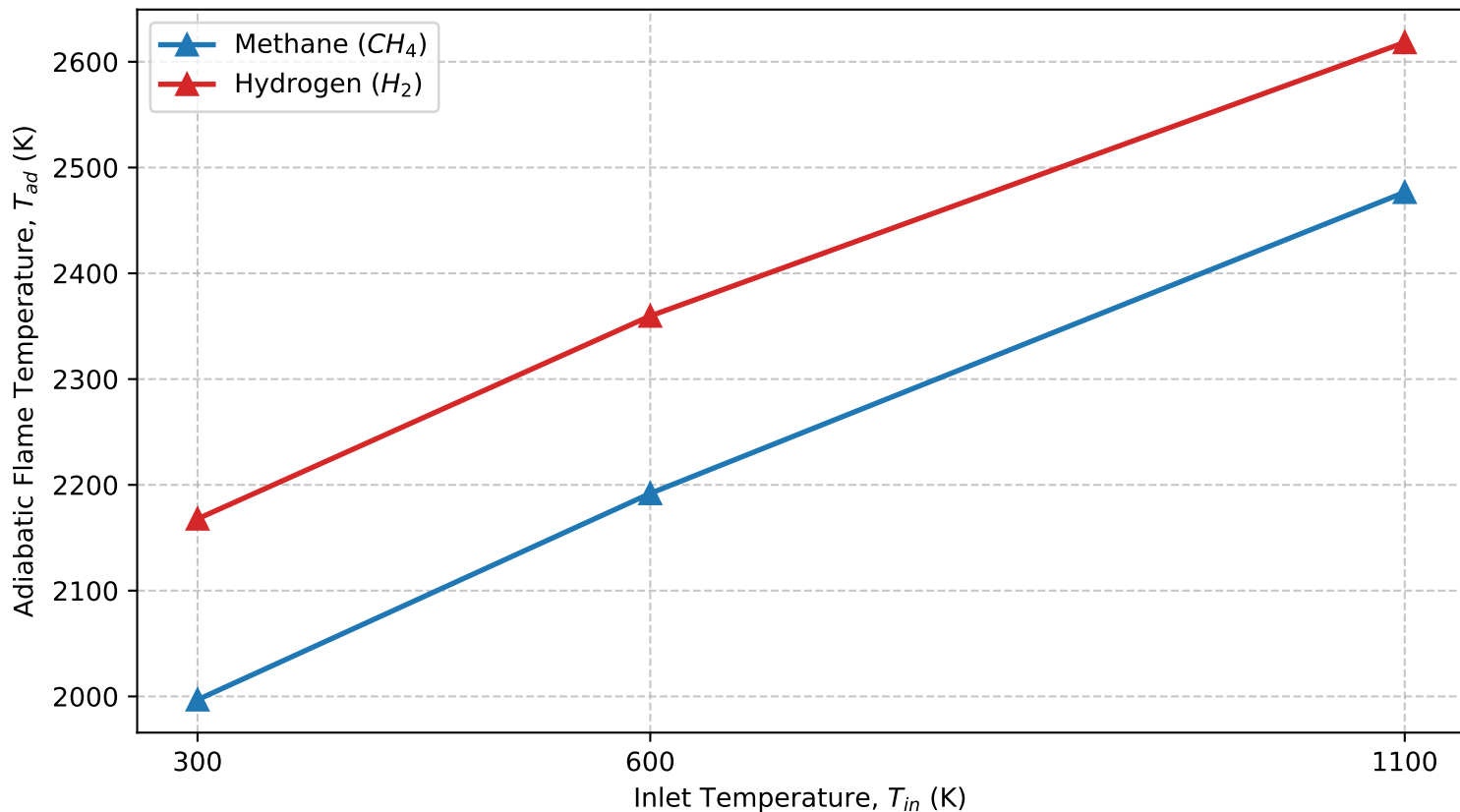
Adiabatic Flame Temp vs Inlet Temperature (Baseline: \phi=0.8 , P=1 bar)
