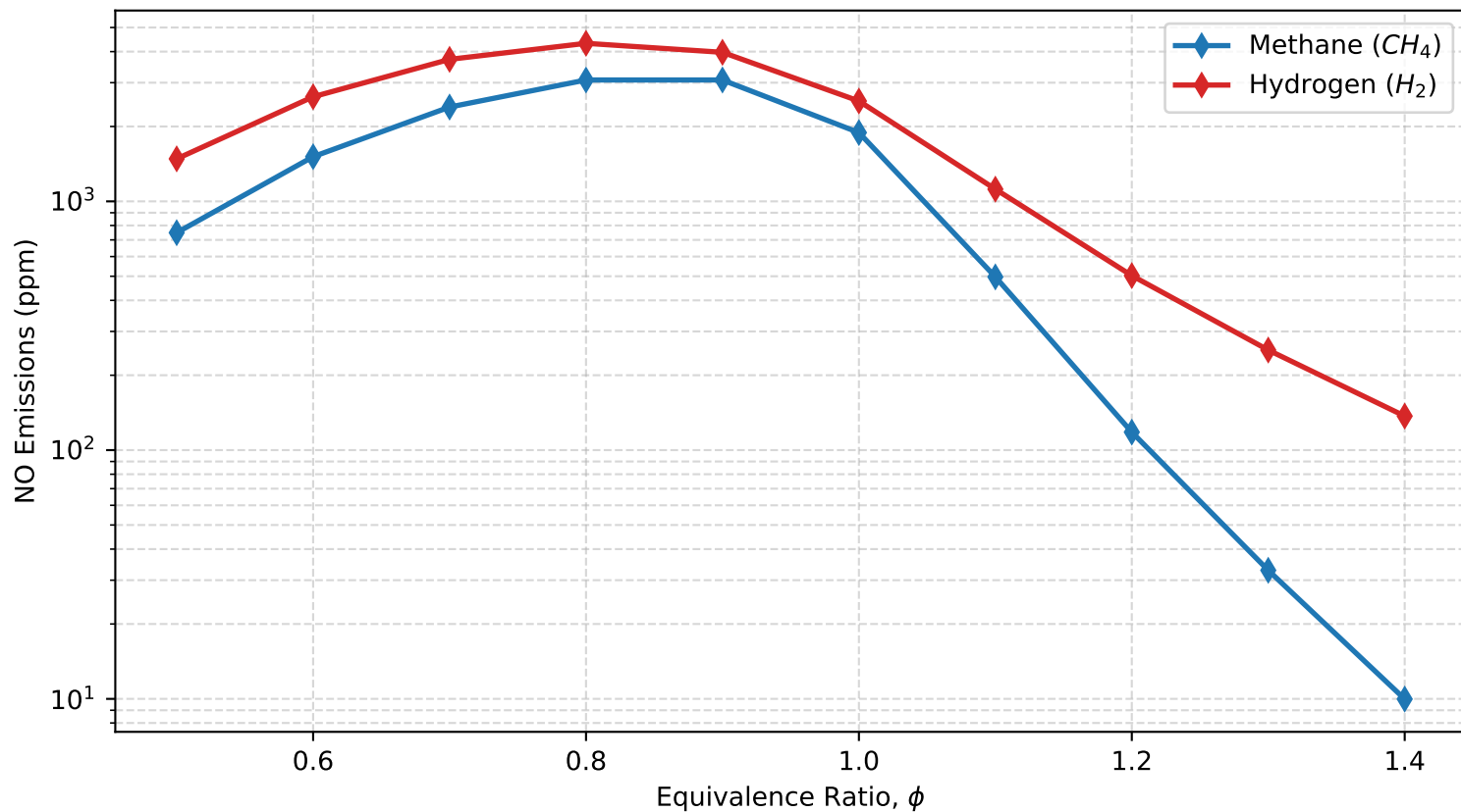
Equilibrium NO Emissions vs Equivalence Ratio (Baseline: T_{in}=300\text{K} , P=1\text{ bar} )
