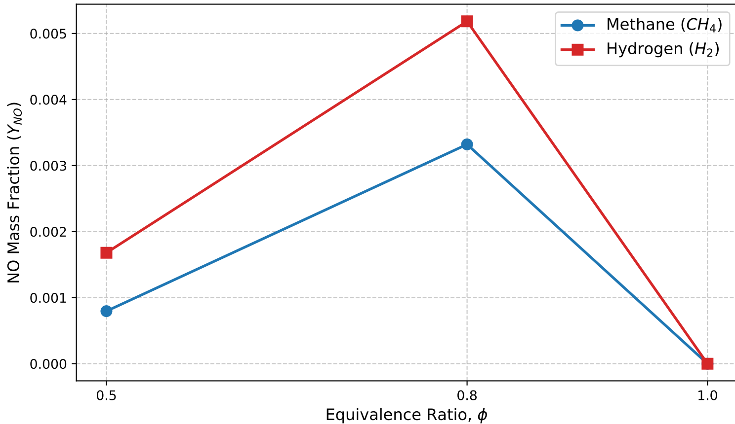
NO Mass Fraction as a function of \phi
