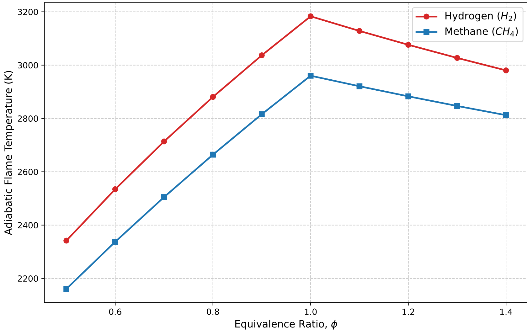
Complete Combustion T_{ad} at T_{in} = 1100 K
