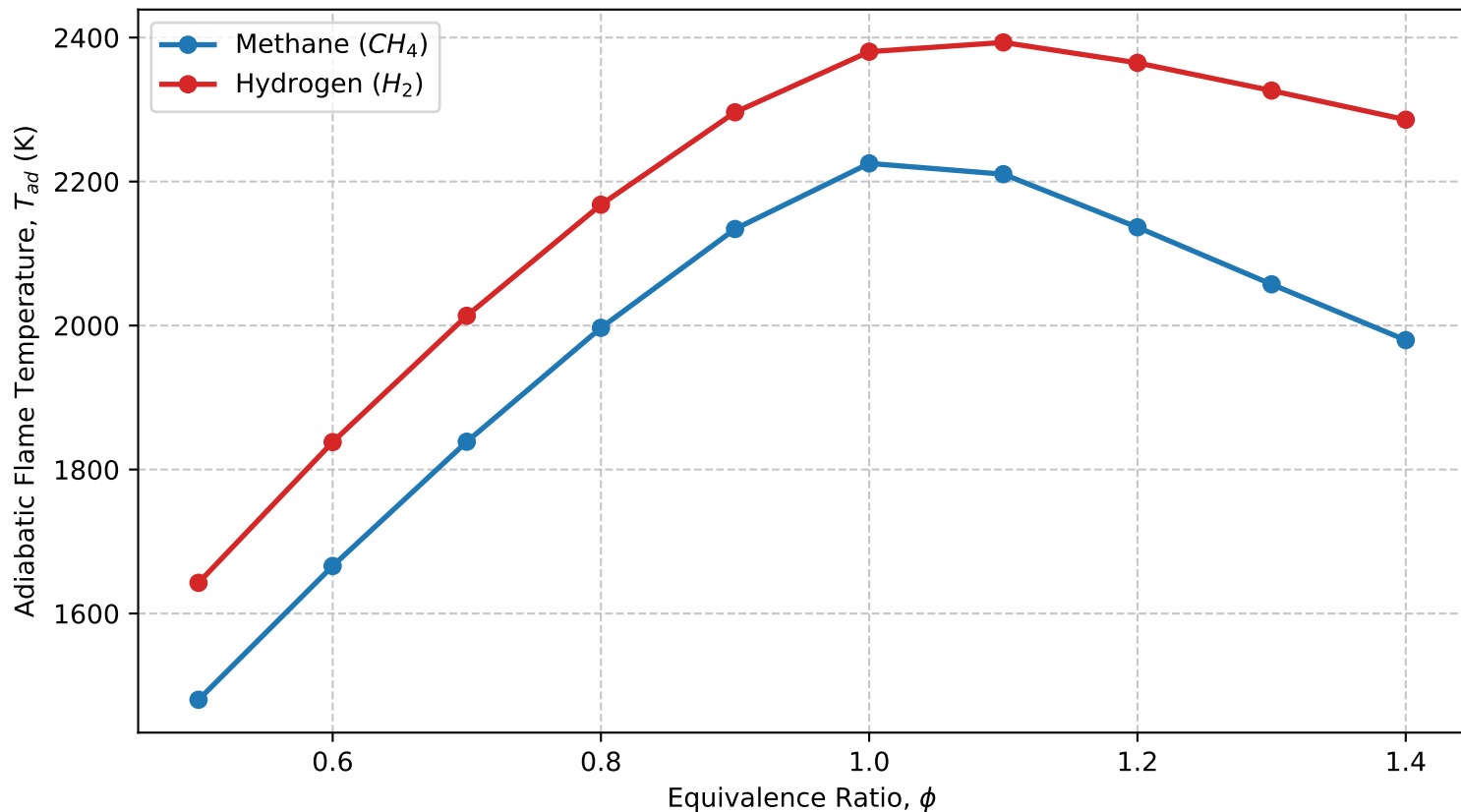
Adiabatic Flame Temp vs Equivalence Ratio (Baseline: T_{in}=300\text{K} , P=1\text{ bar} )
