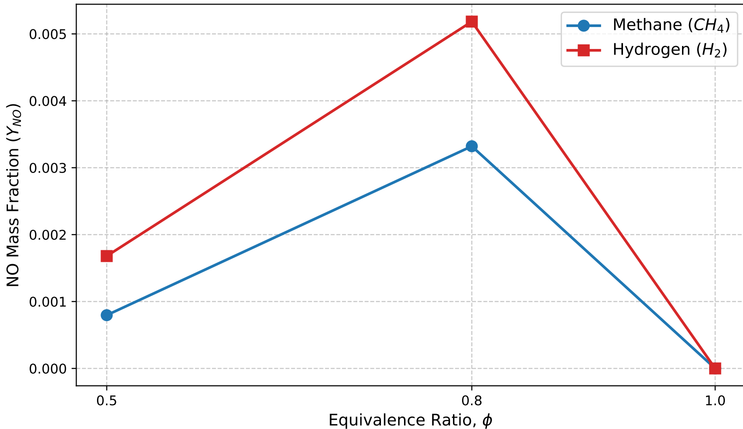
Two-Step Hand Calculation: NO Mass Fraction vs \phi
