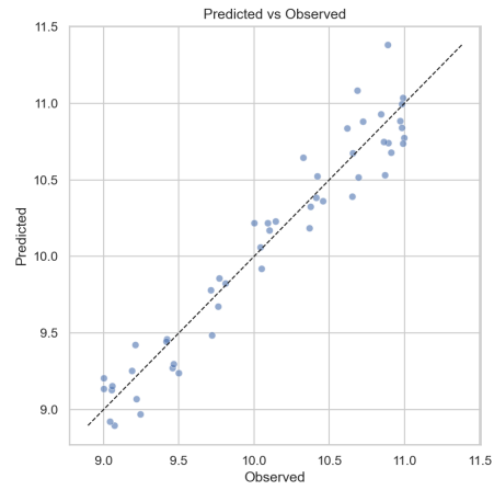
Fig. 3. Predicted against observed reservoir water level values. The alignment with the diagonal illustrates the consistent accuracy of the trained XGBoost.
