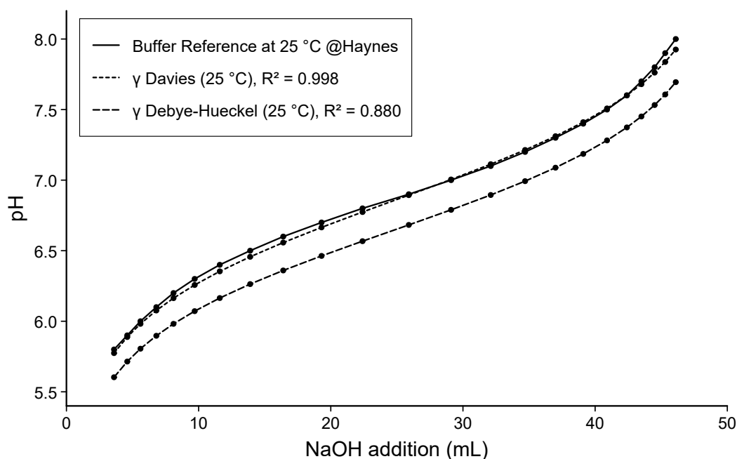
Figure 4.1: Comparison of 50 mL of 0.1 mol L -1 KH 2 PO 4 + x mL of 0.1 mol L -1 NaOH (25 °C).
