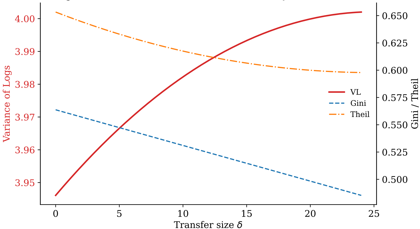
VL transfer-principle violation Progressive transfer from income 100 to 50 in y = (1, 2, 50, 100)
