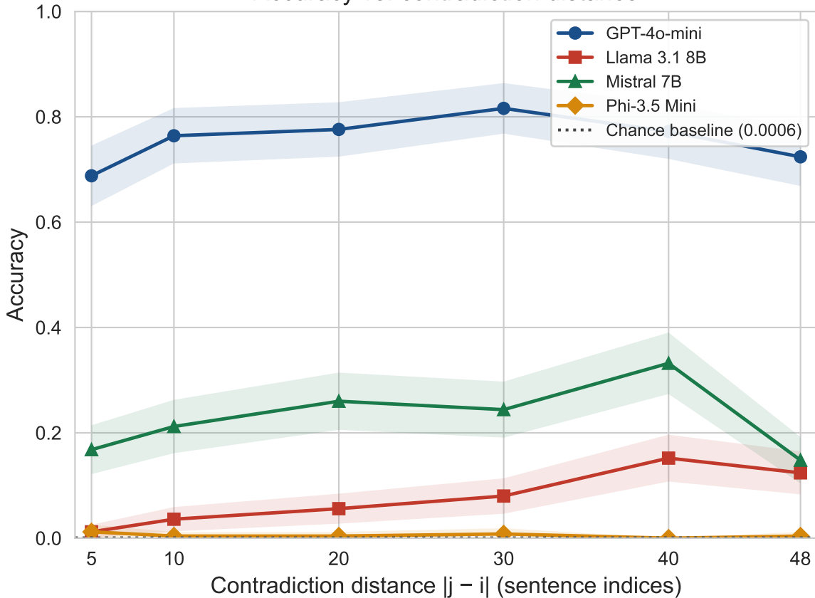
Accuracy vs. contradiction distance
