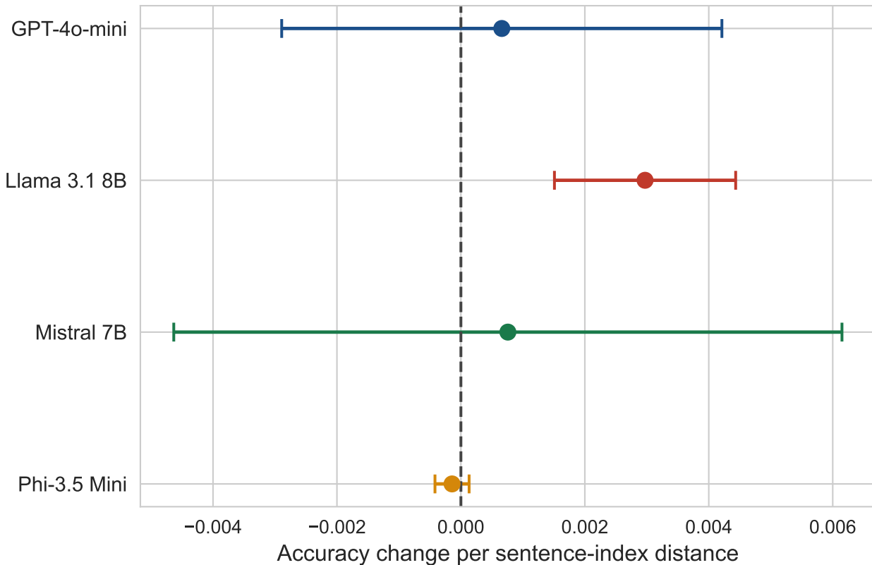
Distance-degradation slope by model
